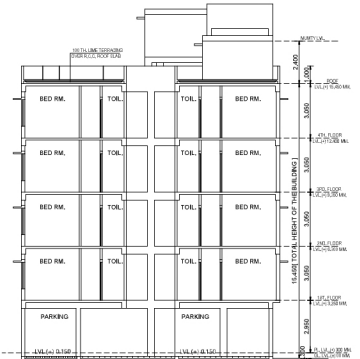
SECTION AT B-B'
